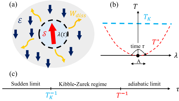
FIG. 1. (a) System \mathcal{S} and environment \mathcal{E} are coupled but share a conserved charge. In a quantum dot setup, the dot spin (red) can be flipped with a compensating spin flip of an electron in the lead (blue). We consider the dissipated work, due to a weak perturbation \lambda(t) such as a magnetic field, ramped in a finite time \tau . (b) Multichannel Kondo systems exhibit quantum critical physics and universality in the intermediate regime T^* < T < T_K , where T_K is the Kondo temperature and T^* \rightarrow 0 at the QCP. (c) We obtain the full, universal crossover from sudden-quench to the adiabatic limit, including the intermediate KZ regime.
