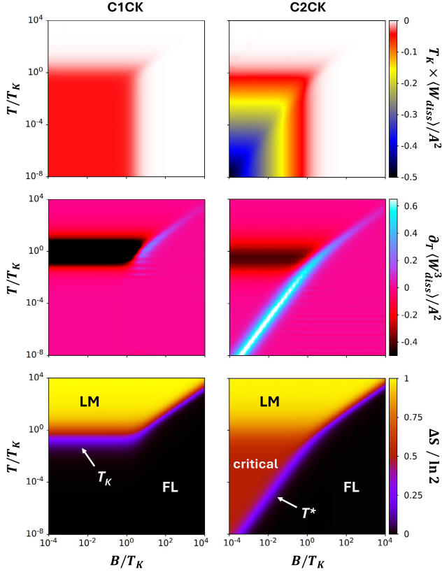
FIG. 3. Universal work statistics phase diagrams in the (T/T_K, B/T_K) plane for the sudden-quench limit, comparing the C1CK model (noncritical, left panels) with the C2CK model (critical, right panels). The expected dissipated work \langle W_{\text{diss}} \rangle in the top row panels shows divergent behavior on approaching the QCP for B \ll T_K and T \ll T_K in the C2CK model (but saturation for C1CK) consistent with interpretation as a susceptibility. Middle row panels for \partial_T \langle W_{\text{diss}}^3 \rangle show the appearance of the critical scale T^* in the C2CK model, reflected also in the thermodynamic entropy \Delta S shown for reference in the bottom row panels (regimes labeled by their RG fixed points). Note that \langle W_{\text{diss}} \rangle and \Delta S are connected by a Maxwell relation. Results obtained by NRG for J = 0.08D .
