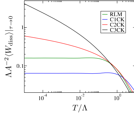
FIG. 4. In the sudden-quench limit \tau \rightarrow 0 , the dissipated work \langle W_{\text{diss}} \rangle in LR is proportional to a susceptibility; see Eq. (9). At low temperatures, \langle W_{\text{diss}} \rangle thus saturates to a finite constant for RLM and C1CK, but it diverges for critical systems like C2CK and C3CK in a way that is characteristic of the QCP. Here, \Lambda = \Gamma for RLM and T_K for CMCK. We set B = 0 .
