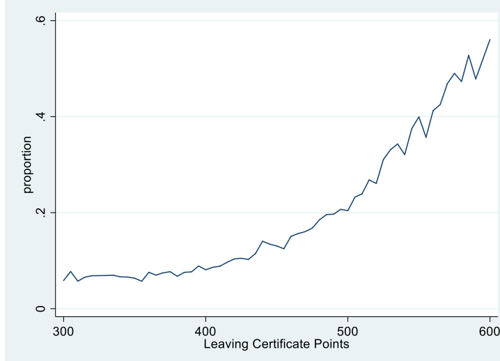
Figure 3: Leaving Certificate Points and Proportion of Completers Obtaining a Great Degree
